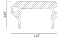
Frosted channel endcap - wired end
